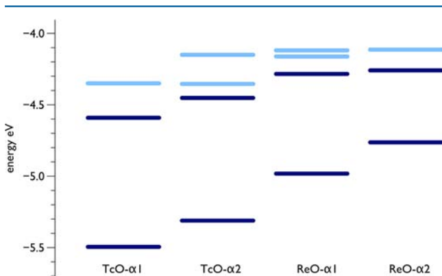
Figure 11. Graphical comparison of the HOMO–LUMO gap extracted from electrochemistry experiments at pH 1 for K_{7-n}H_n[Tc^V O(\alpha_1-P_2W_{17}O_{61})]^{7-} , K_{7-n}H_n[Tc^V O(\alpha_2-P_2W_{17}O_{61})]^{7-} , K_{7-n}H_n[Re^V O(\alpha_1-P_2W_{17}O_{61})]^{7-} , and K_{7-n}H_n[Re^V O(\alpha_2-P_2W_{17}O_{61})]^{7-} . The dark blue lines represent the HOMO and LUMO and the light blue lines represent the nearest W redox processes.
