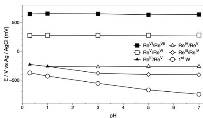
Figure 10. Reduction potentials of 10^{-3} M [\text{Re}^{\text{V}}\text{O}(\alpha_2\text{-P}_2\text{W}_{17}\text{O}_{61})]^{7-} as a function of pH.
