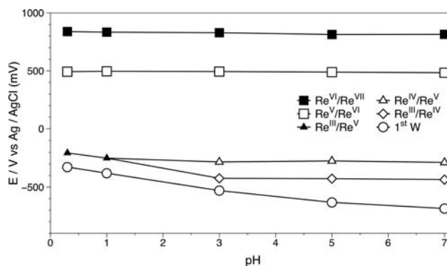
Figure 8. Reduction potentials of 10^{-3} M [\text{Re}^{\text{V}}\text{O}(\alpha_1\text{-P}_2\text{W}_{17}\text{O}_{61})]^{7-} as a function of pH.
