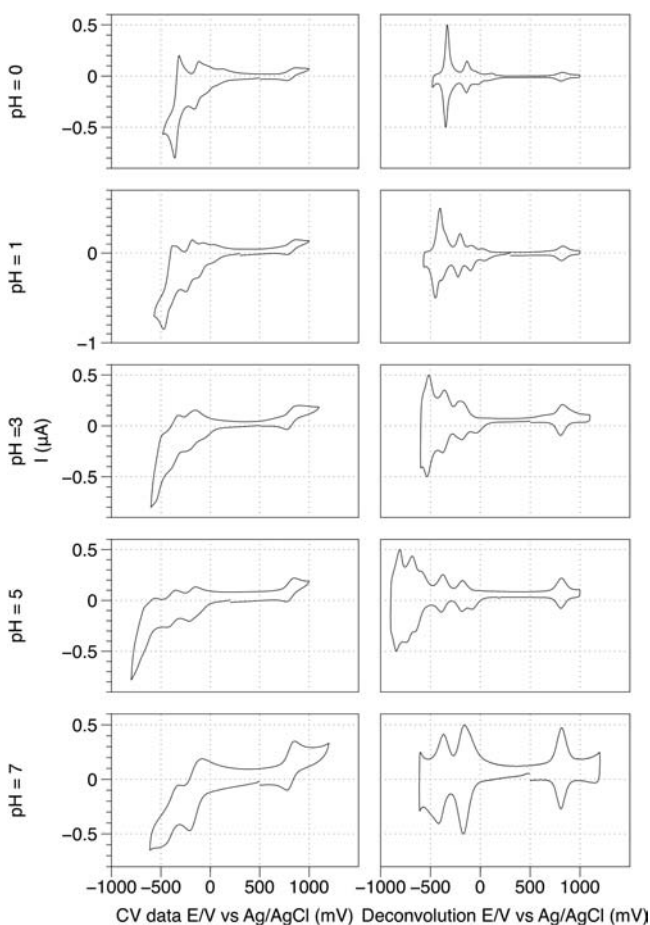
Figure 5. CV data of K_{7-n}H_n[Tc^V O(\alpha_2-P_2W_{17}O_{61})] as a function of pH. Electrolyte, 0.5 M Na_2SO_4 . Working electrode, glassy carbon, auxiliary electrode, platinum wire, and reference electrode, Ag/AgCl. Scan rate 10 mV/s.
